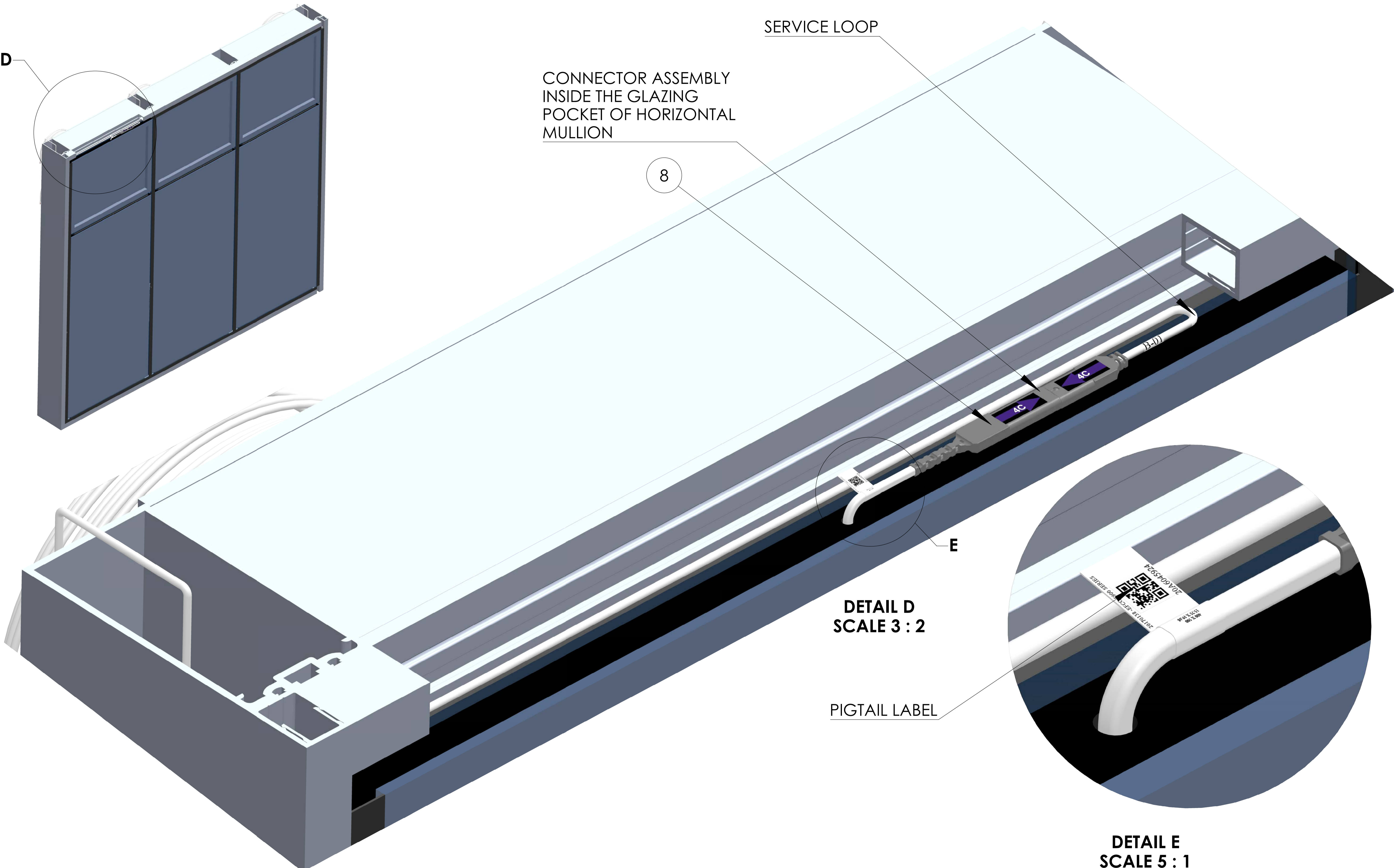
⑧ - CONNECTOR ASSEMBLY
